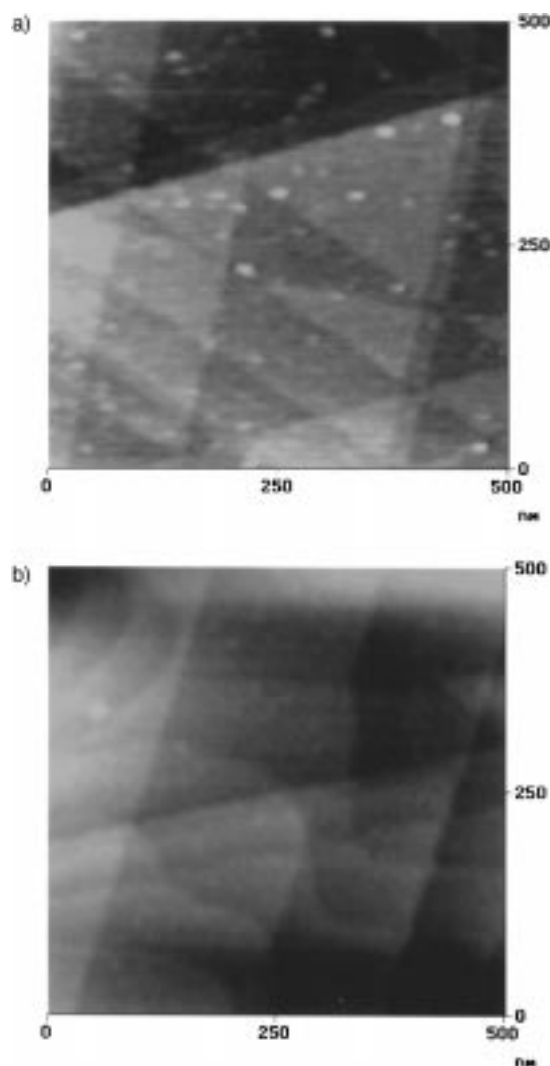
Figure 1. AFM height image (tapping mode) of the [\text{D}_{21}] decanethiol monolayer on Au(111) after treatment with a solution of a) metallogen-dendrimer \text{MG}_2 and b) reference compound ( \text{G}_{2\text{py}} ). (Color scale from dark to white: Z = 10 \text{ nm} ).
